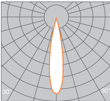
Zoomable Distribution 10°
