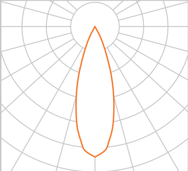
Medium Distribution 25°
