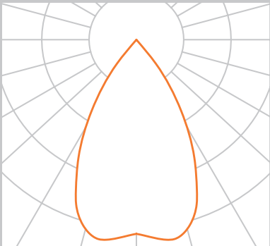
Batwing Distribution 60°
