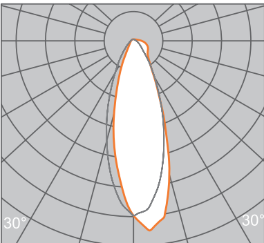
Wallwash Distribution
